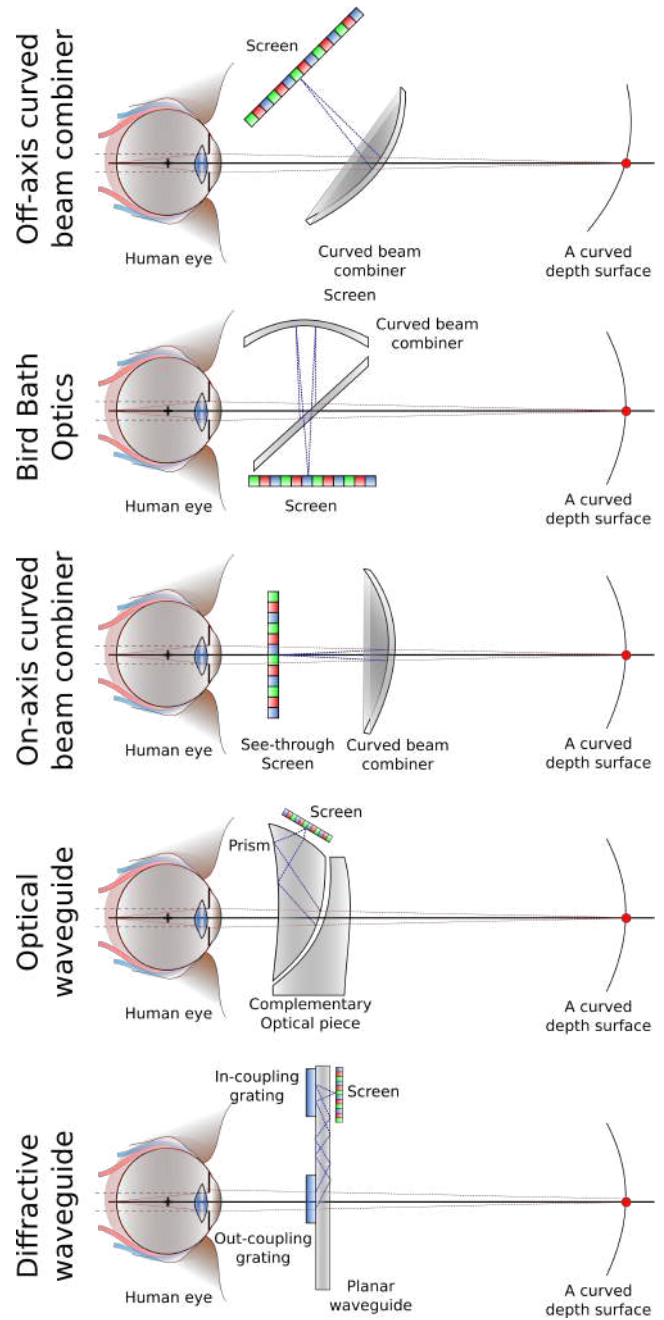
Figure 4: Diagrams showing various optical layouts for near-eye displays. From top to bottom: off-axis curved beam combiner; bird bath optics, on-axis curved beam combiner, optical waveguide, and diffractive waveguide layouts.
