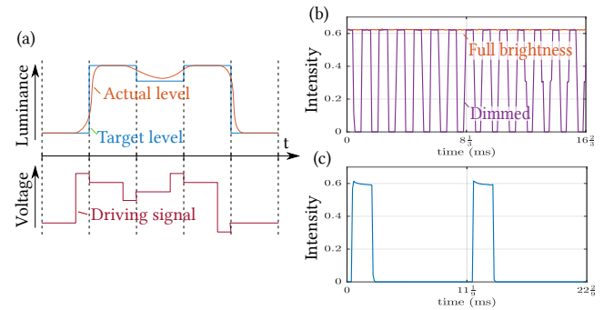
Figure 3: (a) Delayed response of an LCD, driven by a signal with overdrive. The plot is for illustrative purposes and does not represent measurements. (b) Measurement of an LCD (Dell Inspiron 17R 7720) at full brightness and when dimmed, showing all-white pixels in both cases. (c) Measurement of an HTC Vive display showing all-white pixels. Measurements taken with a 9 kHz irradiance sensor.
