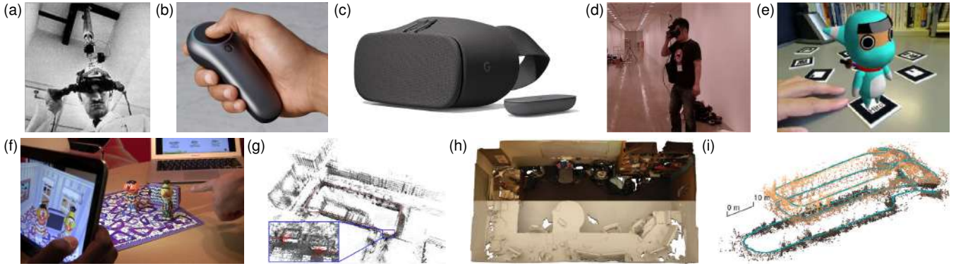
Figure 7: Example uses of the tracking technologies discussed in Section 4.1: (a) Sutherland’s ‘Sword of Damocles’ mechanical tracker (1968) [Sut68]; (b) the Magic Leap One Controller (2018) uses magnetic tracking [BLW* 17]; (c) Google Daydream View (2017) uses inertial tracking for 3-DoF localisation of headset and controller; (d) ultrasonic tracking for room-scale 6-DoF localisation [SAP* 16]; (e) marker-based optical tracking using ARToolkit [KB99]; (f) model-based optical tracking using Vuforia; (g) SLAM-based tracking using direct sparse odometry [EKC18]; (h) depth-based tracking using BundleFusion [DNZ* 17]; and (i) visual-inertial odometry [LLB* 15] as a hybrid technique combining optical and inertial tracking.
