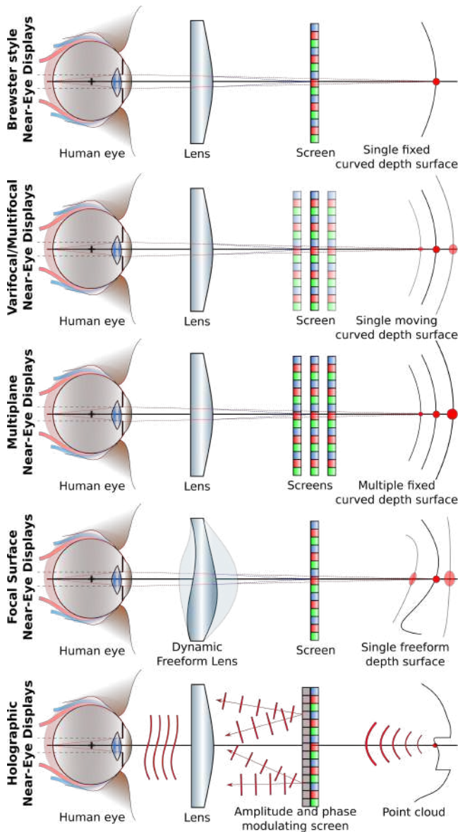
Figure 5: Diagrams comparing generic optical layouts for various different types of accommodation-supporting near-eye displays with a traditional Brewster-style near-eye display layout [Bre56]. Accommodation-supporting near-eye displays can be classified as varifocal/multifocal, multiplane, focal surface, and holographic near-eye displays.
